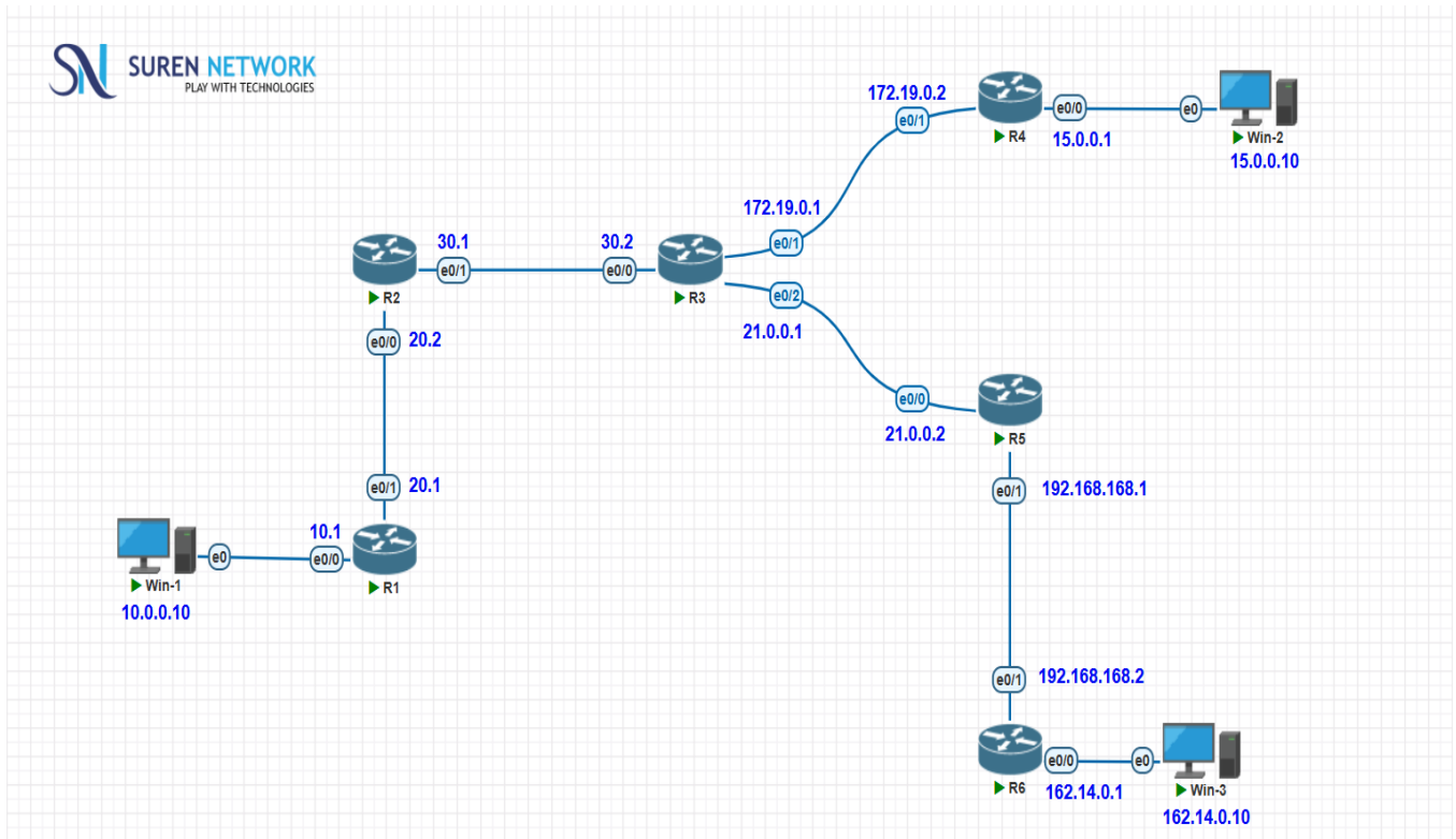
Figure 1: Network topology used for the connectivity testing lab.
